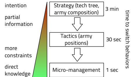
Fig. 1. Gameplay levels of abstraction for RTS games, compared with their level of direct (and complete) information and orders of magnitudes of time to chance their policies.
