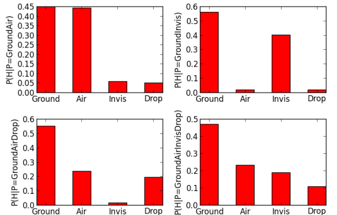
Fig. 4. P(H|HP) for varying values H and for different values of P (derived from inferred TT ), for Protoss in PvT.
