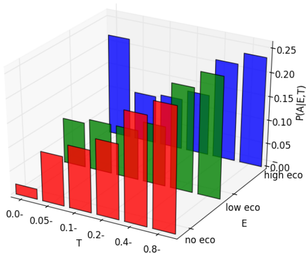
Fig. 5. P(A) for varying values of E and T , summed on the other variables, for Terran in TvT.
